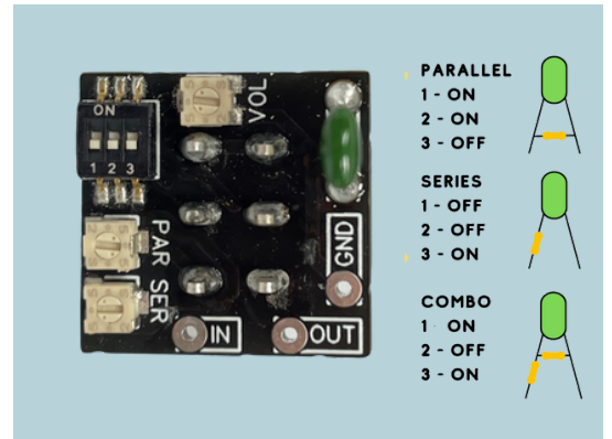
fig.2. Board layout and settings for the variable trim pots
