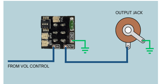
fig.1. Wiring Diagram
