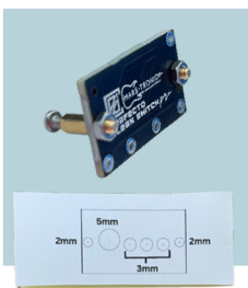
fig.4. Clean Switch with mounting feet attached and drill template sticker.
