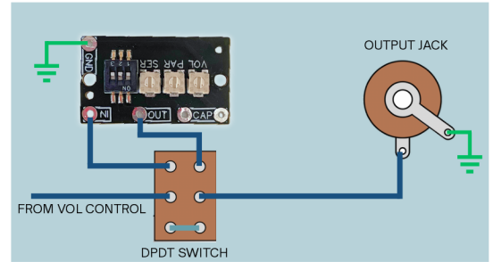
fig.1. Wiring Diagram
